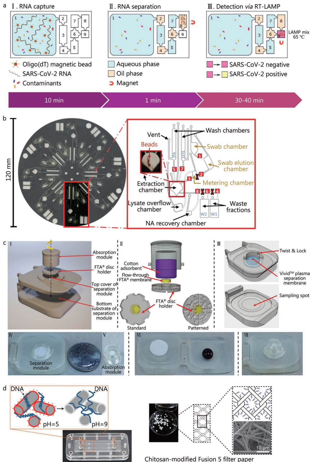
Fig. 2 Magnetic- and porous material-based devices.
