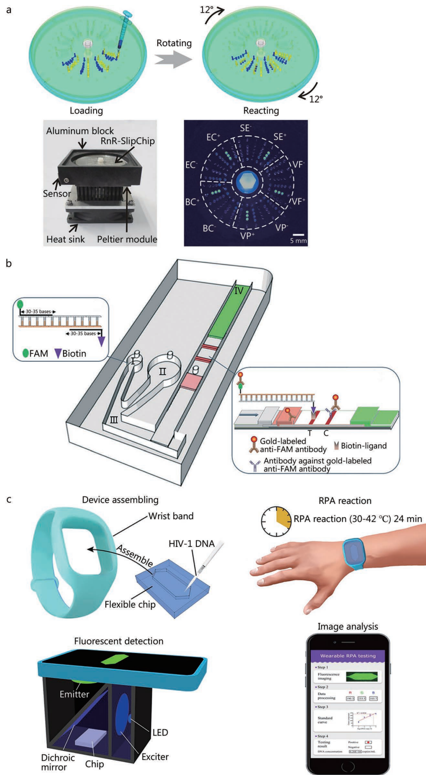
Fig. 4 Isothermal amplification in point-of-care testing (POCT).
